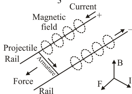
Schematic diagram of a railgun
